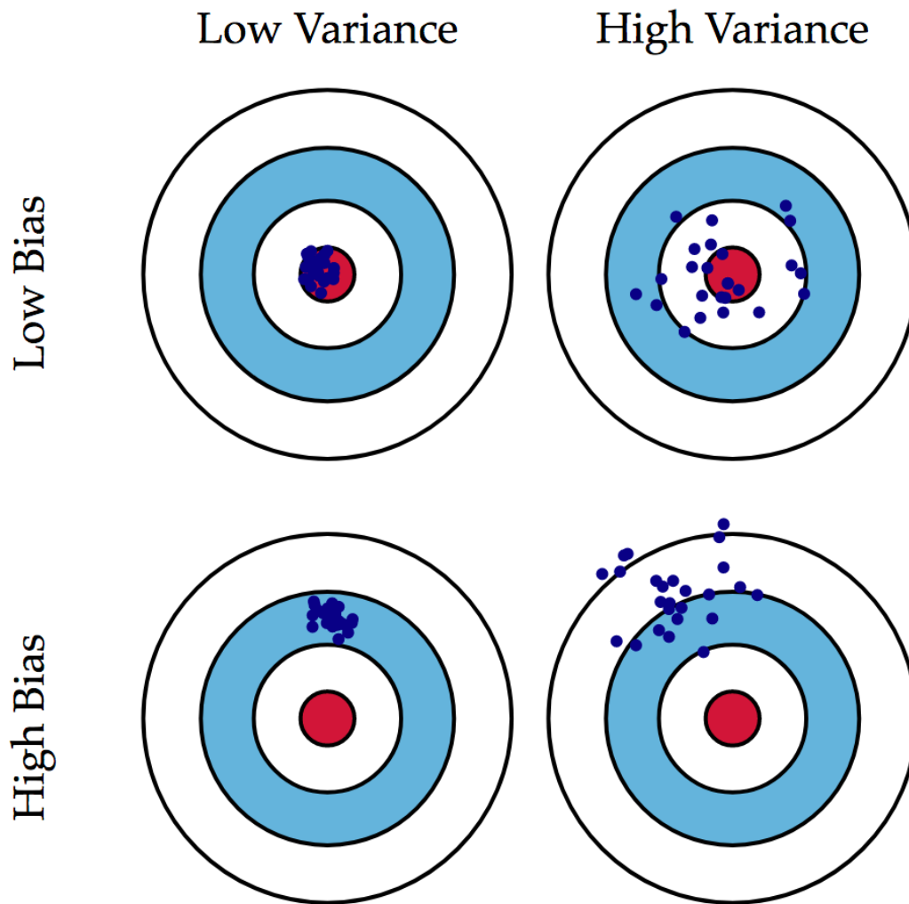
Bias vs. Variance
